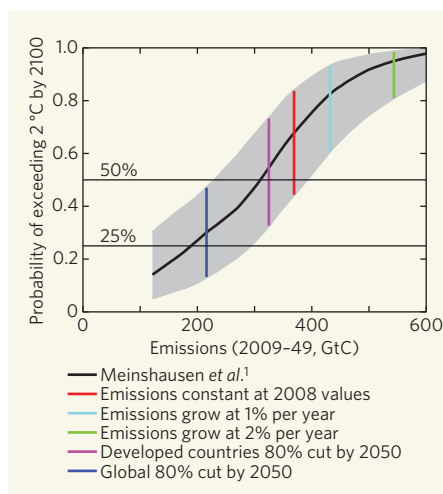
Figure 1 | The 2 °C lottery. The black line shows the probability of the peak global mean temperature exceeding 2 °C above pre-industrial levels before the year 2100 as a function of the integrated emissions from 2009 to 2049. The graph is adapted from the base case of Meinshausen et al. 1 , including uncertainty ranges. Also shown are the cumulative emissions under various scenarios. Red, emissions constant at 2008 values until 2050. Light blue, growth in emissions continues at 1% per year until 2050 and then falls rapidly. Green, growth in emissions continues at 2% per year until 2050 and then falls rapidly. Purple, an 80% cut in emissions by 2050 (linearly applied, starting in 2010) from developed countries only, while developing-country emissions continue to grow at 1% per year. Dark blue, an 80% cut in emissions by 2050 from all countries.
