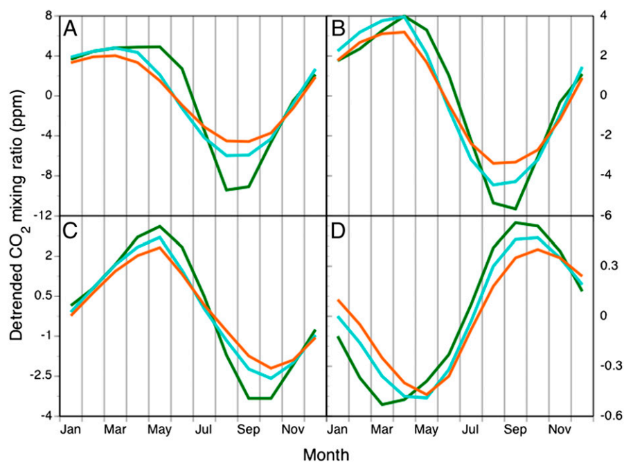
Fig. 4. Annual cycles of atmospheric \text{CO}_2 mixing ratio at (A) Alert, Nunavut, Canada ( 82.45^\circ\text{N} ), (B) Terceira Island, Azores, Portugal ( 38.8^\circ\text{N} ), (C) Mauna Loa, Hawaii, United States ( 19.5^\circ\text{N} ), and (D) South Pole, Antarctica. Observation-based estimates are from the GLOBALVIEW- \text{CO}_2 product (43, 44) for years 1988–2004. Model estimates are detrended mean seasonal cycles from 1988 to 2004 from a simulation forced with reanalysis surface weather, historic \text{CO}_2 concentrations, historic nitrogen deposition, and historic land-use changes, and were obtained by impulse response function analysis (19). Results are shown for both the model without a day-length correction to V_{\text{cmax}} (orange line), and with a day-length correction to V_{\text{cmax}} (cyan line).
